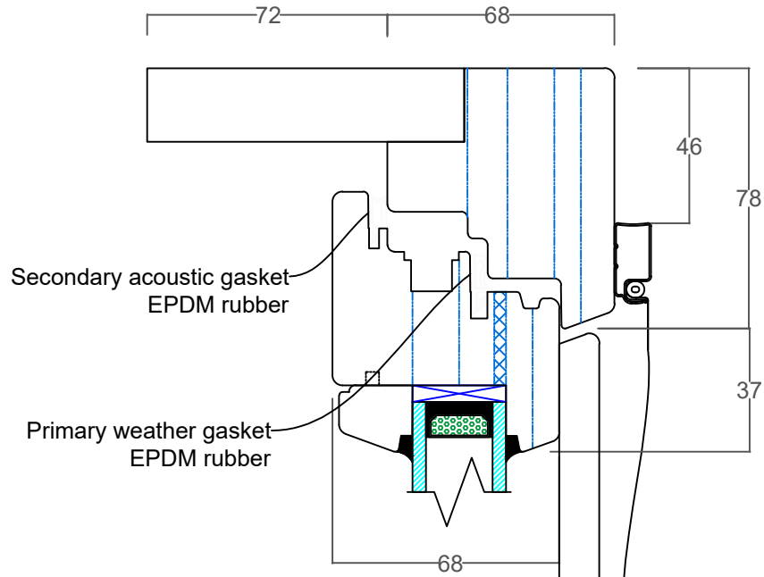
BINQ TILT & TURN WINDOW 140mm INTERNAL REVEAL SECTION DETAIL
